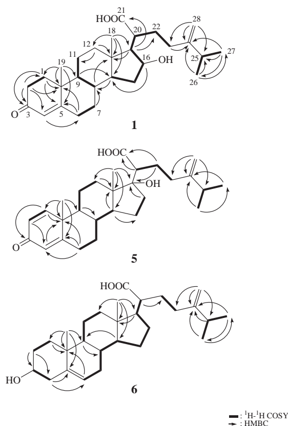
Fig. 1. Selective 1 H- 1 H COSY and HMBC correlations for 1 , 5 , and 6 .
