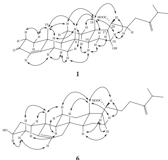
Fig. 2. Selective NOESY correlations for 1 and 6 .
